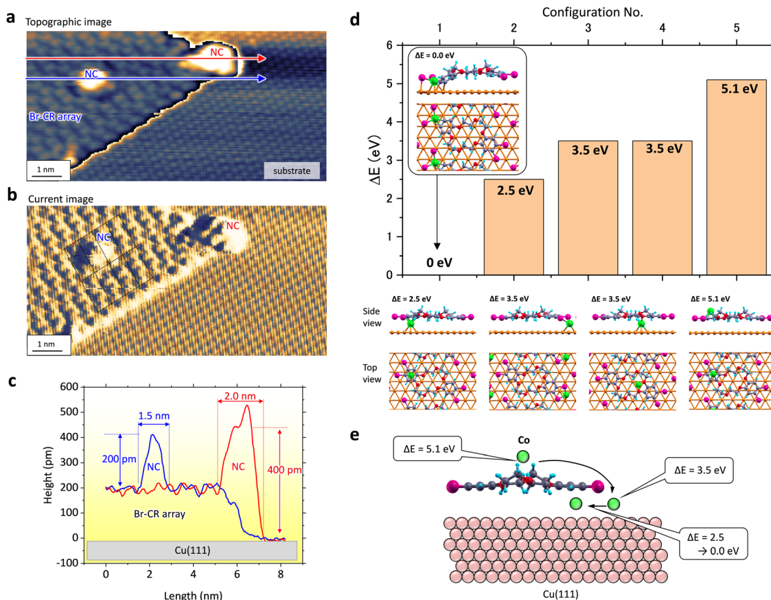
Fig. 3 (a) and (b) Simultaneously obtained STM topographic image and current map at the edge of the BrCR array island, where two Co nanoclusters (NCs) are observed ( 10 \times 5 \text{ nm}^2 , -2 \text{ V} , 10 \text{ pA} ). (c) Height profiles along the red and blue arrows in (a). (d) DFT calculation results of Co atom adsorption into the BrCR/Cu(111) system. Ball-and-stick models of five configurations are shown with Co, Br, O, C, H, and Cu atoms in green, magenta, red, grey, blue, and golden, respectively. Side and top views are shown. The Co atom is placed between Br atoms and the benzene ring (no. 1), below the benzene ring (no. 2), below or outside the Br atoms (no. 3), below the crown ring (no. 4), and above the benzene ring (no. 5). \Delta E denotes the energy value difference from the most stable configuration. (e) DFT calculation suggested a model of how the adsorbed Co atom moved to the stable position.
